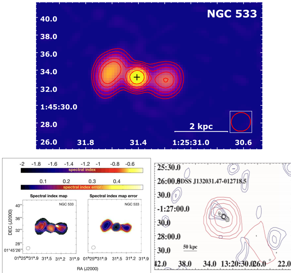
Figure 4.14: Top: The total intensity image of NGC 533 in VLA A configuration at 1–2 GHz and (bottom left) its corresponding in-band spectral index map with measurement uncertainties produced by the multi-term ‘cleaning’ algorithm in CASA. Bottom right: The morphological structure of NGC 533 is similar to the structure in the COMP2CAT source J132031.47-012718.5.
