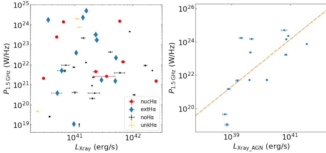
Figure 4.4: Left: Relation between radio power at \sim 1.5 GHz ( P_{1.5\text{GHz}} ) vs. the X-ray luminosity ( L_{X\text{ray}} ) within the 10 kpc from the center of the galaxy shows no correlation. Right: Significant correlation ( r \sim 0.68 , P-value \sim 0.01 ) is seen, when we compare the radio power at \sim 1.5 GHz ( P_{1.5\text{GHz}} ) with the luminosity of the central X-ray point sources ( L_{X\text{ray\_AGN}} ) (Lakhchaura et al. 2018) detected only in a subset of our main sample of early-type galaxies. Error bars on the radio power are mostly smaller than the plotted symbol size. The correlation coefficients and corresponding P-values are given in Table 4.1.
