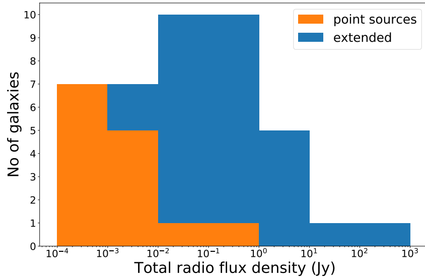
Figure 4.8: The total integrated radio flux density histogram with two morphologically different categories: point sources and extended sources. The fainter sources fall into the point sources category, whereas the brighter galaxies are the extended ones.
