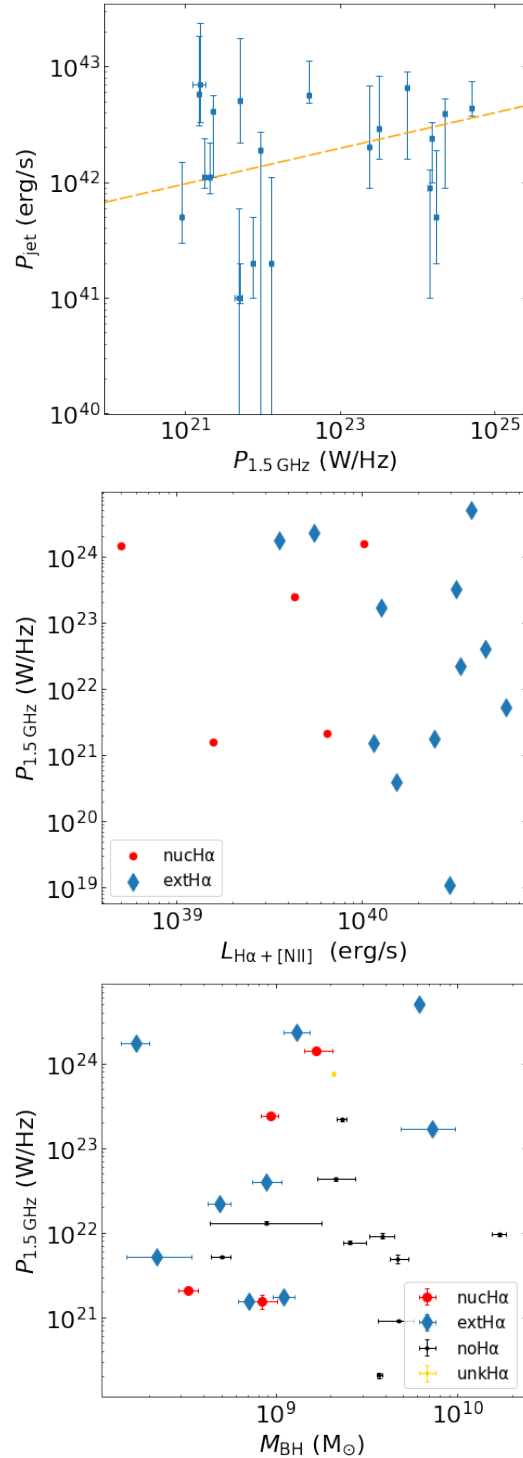
Figure 4.6: Top: Radio power ( P_{1.5\text{GHz}} ) vs. the jet power ( P_{\text{jet}} ) shows a hint correlation ( r \sim 0.46 , P-value \sim 0.04 ). Middle: The \text{H}\alpha + [\text{NII}] luminosity ( L_{\text{H}\alpha + [\text{NII}]} ) vs. radio power ( P_{1.5\text{GHz}} ) relation shows no correlation. Bottom: Likewise, no correlation was found between the radio power ( P_{1.5\text{GHz}} ) and the supermassive black hole mass ( M_{\text{BH}} ). The nuclear (nucH \alpha ), extended (extH \alpha ), undetected (noH \alpha ) and unknown (unkH \alpha ) \text{H}\alpha + [\text{NII}] emission are distinguished. The correlation coefficients and corresponding P-values are given in Table 4.1. Error bars on the radio power are mostly smaller than the plotted symbol size.
