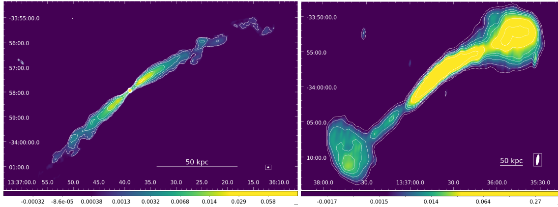
Figure 6.1: VLA total intensity images of IC 4296 at 1.5 GHz. Left: the A configuration image shows that the surface brightness of jets decreases as a function of radius, although we also see re-brightening in the radio plumes at \sim 10 kpc from the nucleus. The restoring beam size is 3.94'' \times 3.26'' and is shown in the bottom right corner. Right: the D configuration image revealed well-confined radio lobes extending up to almost 300 kpc from the central regions of IC 4296, previously reported by Killeen et al. (1986b). The restoring beam is 90.15'' \times 23.02'' and is shown in the bottom-right corner. The contour levels are at [-1, 1, 2, 4, 8, 16] \times 5 rms noise, with corresponding rms noise of 0.06 \text{ mJy beam}^{-1} and of 0.2 \text{ mJy beam}^{-1} for VLA A and D configuration data, respectively.
