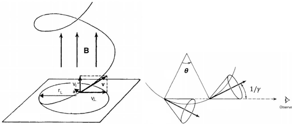
Figure 1.6: Left: Scheme of the helical motion of a relativistic particle with labelled velocity components (parallel, v_{\parallel} , and perpendicular, v_{\perp} ), acceleration, a , magnetic field, B , perpendicular to the main plane, Larmor radius, r_L , (Carroll & Ostlie 2006). Right: The radiation from the relativistic electron gets visible only for a short time and a small fraction \sim 1/\gamma of electron's orbit, when the beam is pointed at our line of sight (Rybicki & Lightman 1979).
