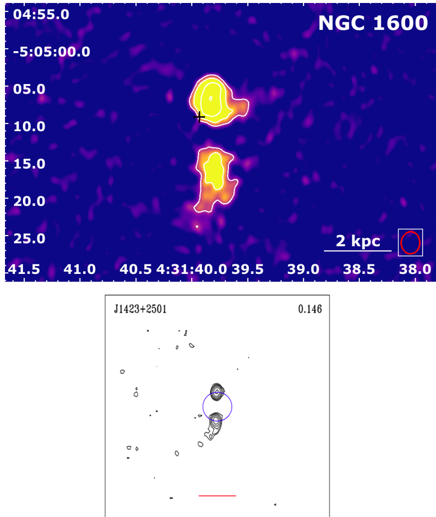
Figure 4.15: Top: The total intensity image of NGC 1600 in VLA A configuration at 1–2 GHz has a morphology resembling the FR II radio source J1423+2501 from the FRIICAT catalog (Capetti et al. 2017b) ( bottom ).
