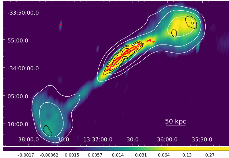
Figure 6.2: VLA D configuration radio map at 1.5 GHz overlaid with the TGSS radio contours at 153 MHz (in black), VLA A configuration contours at 1.5 GHz (in red), and the GLEAM radio maps at 154–162 GHz (in white). Contours levels were created at [-1, 1, 2, 4, 8, 16] \times 5 rms noise for the TGSS, GLEAM, VLA A configuration data with corresponding rms noise of 3, 0.12, and 0.06 \text{ mJy beam}^{-1} .
