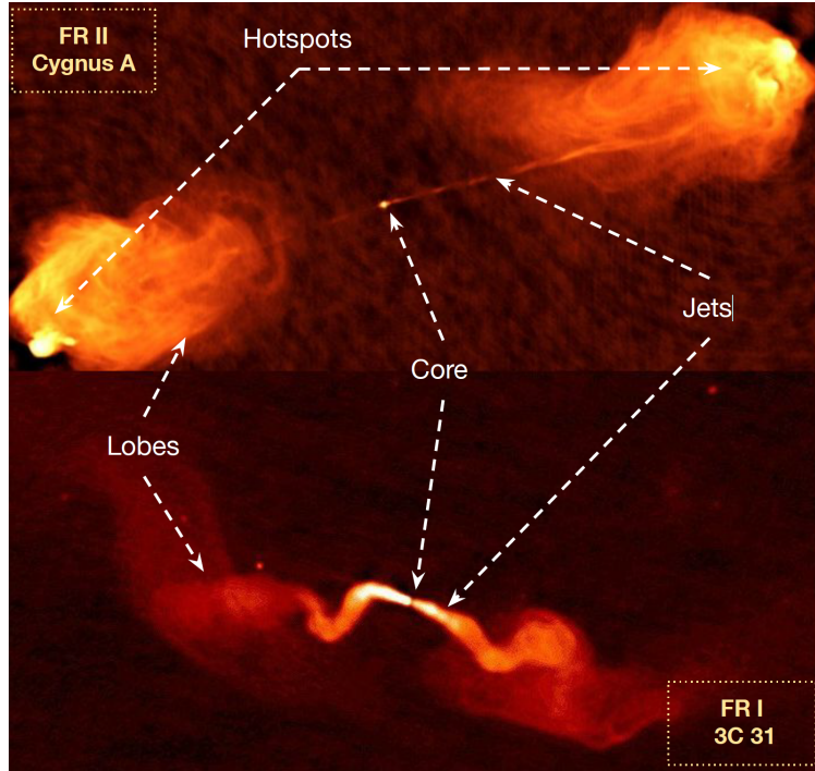
Figure 1.4: Individual components of radio jets for low (FRI) and high (FRII) power radio sources (see discussion in Section 1.3.1). Credit to: NRAO/AUI (Galaxies/) by R.Laing, A. Bridle, R. Perley, L. Feretti, G. Giovannini, and P. Parma & NRAO/AUI by Chris Carilli.
