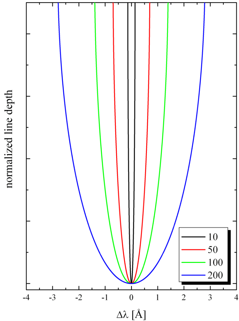
Rotational profile
